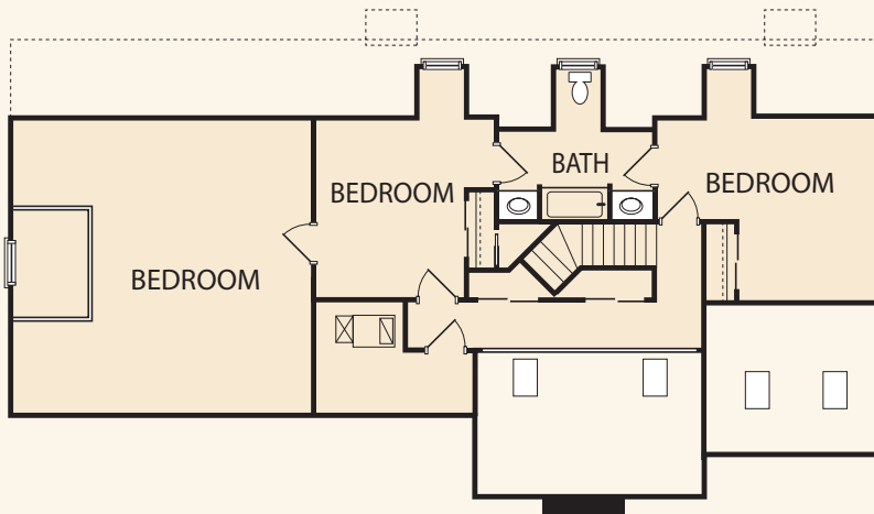
Model GS-4 BEDROOM: 13' x 14' BEDROOM: 11'-6" x 14' BATH: 11'-7" x 6'-9"
